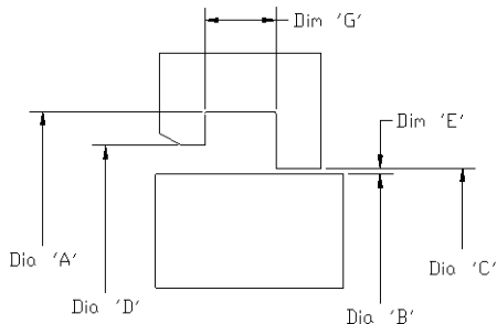
Rod Seal / Wiper
