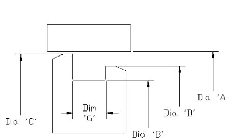
Piston Seal
